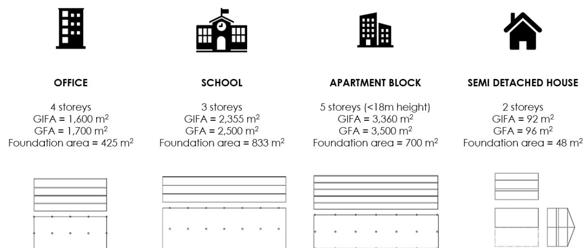
Figure 2-1 - Building Typologies
