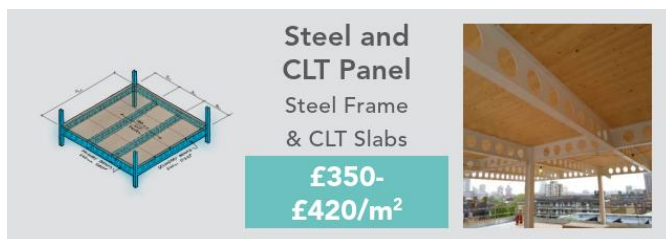
Figure 3-11 – Typical frame construction cost steel frame with CLT panel slabs
